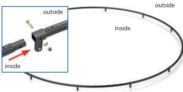
fig. 1: Trampoline frame assembly
