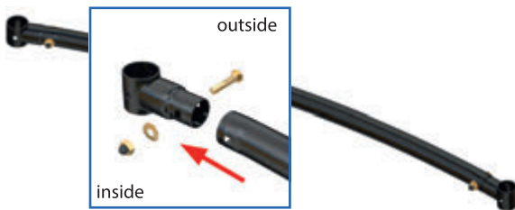
fig. 2: Assembly of the feet
